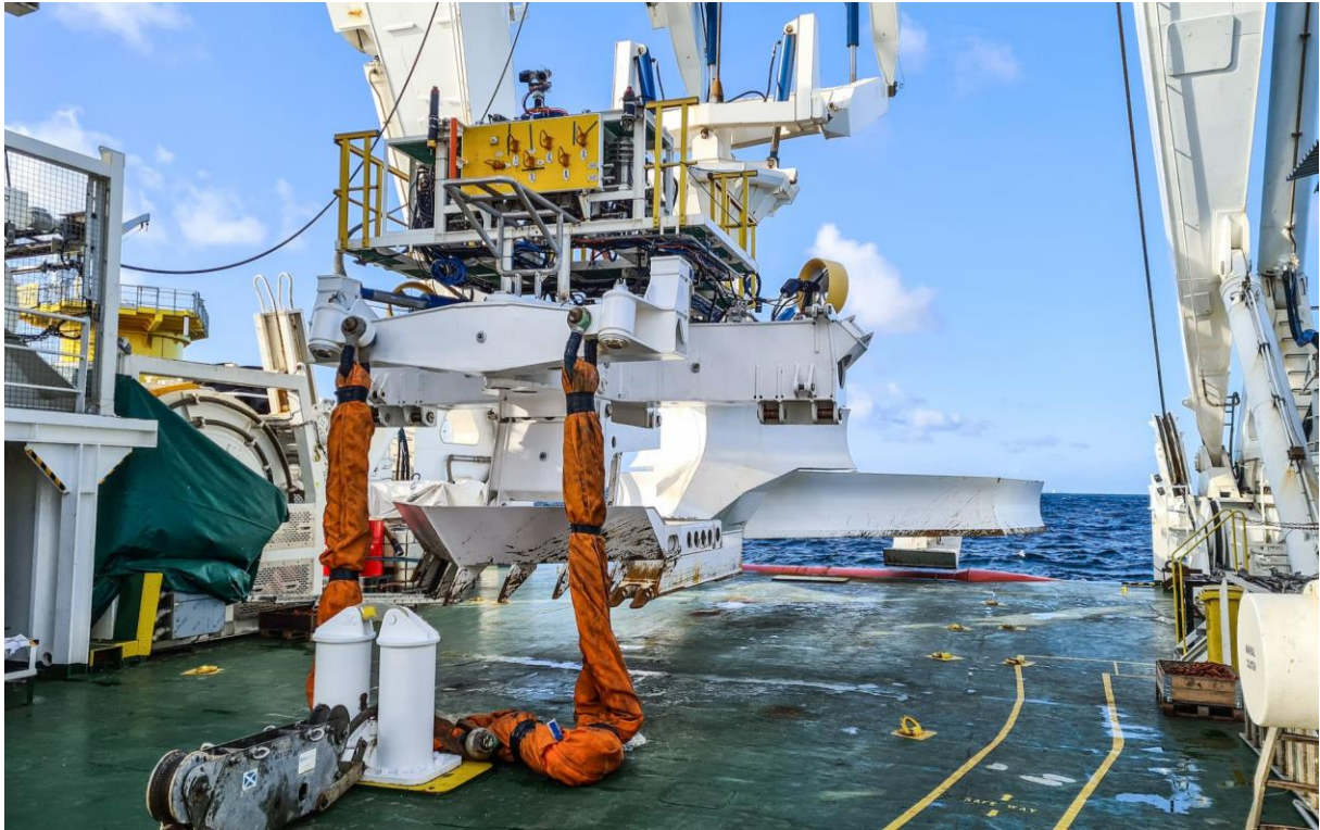
Figure 22: Asso Subsea's Multi-Functional Plough
