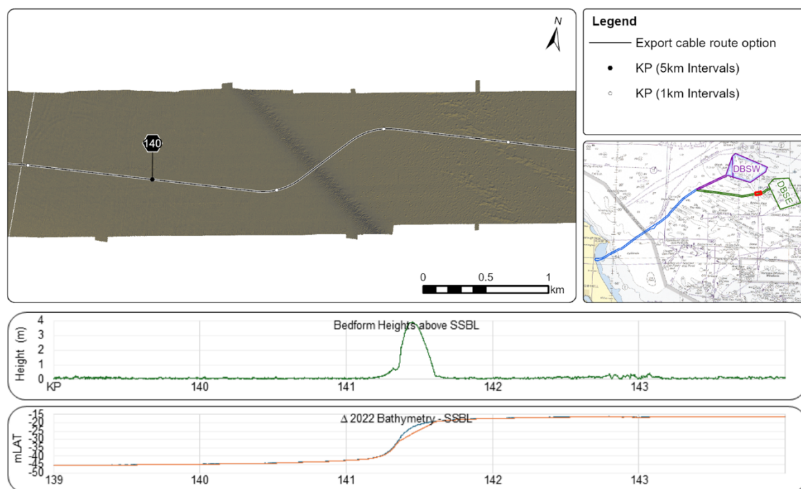
Figure 26: Bedform Heights and Seabed Delta (Route C; KP139 – KP144)
