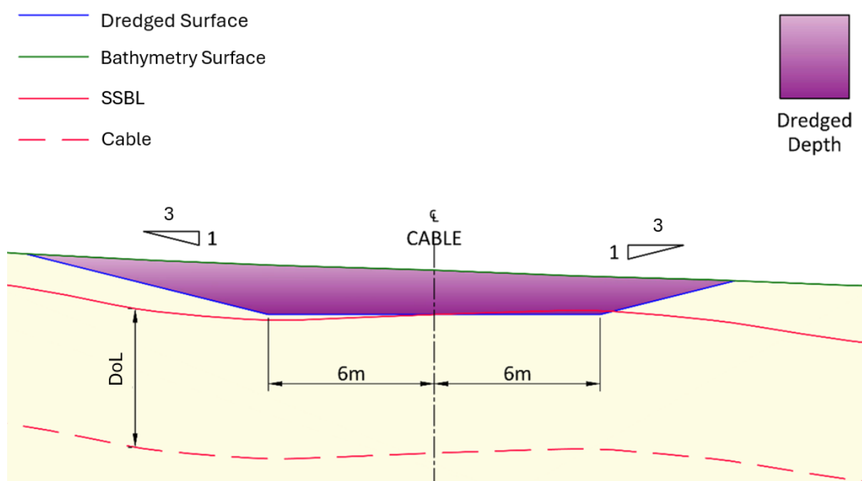
Figure 32: Typical Dredging Cross Section
